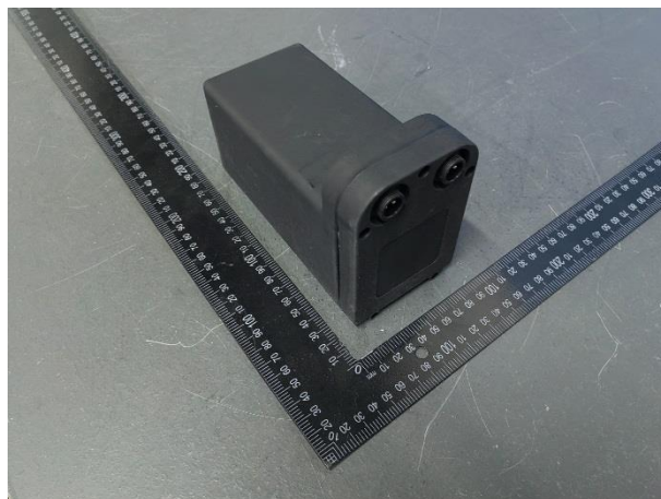
Battery/电池 (DJ-2410 24V 10Ah 240Wh)
